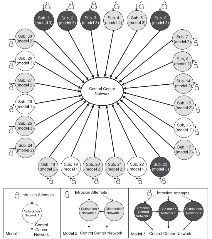
Fig. 10. Case Setup for IEEE 30 Bus System
