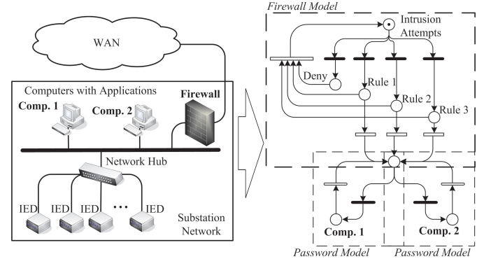
Fig. 6. Formulation of Cyber-Net with Firewall and Password Models
