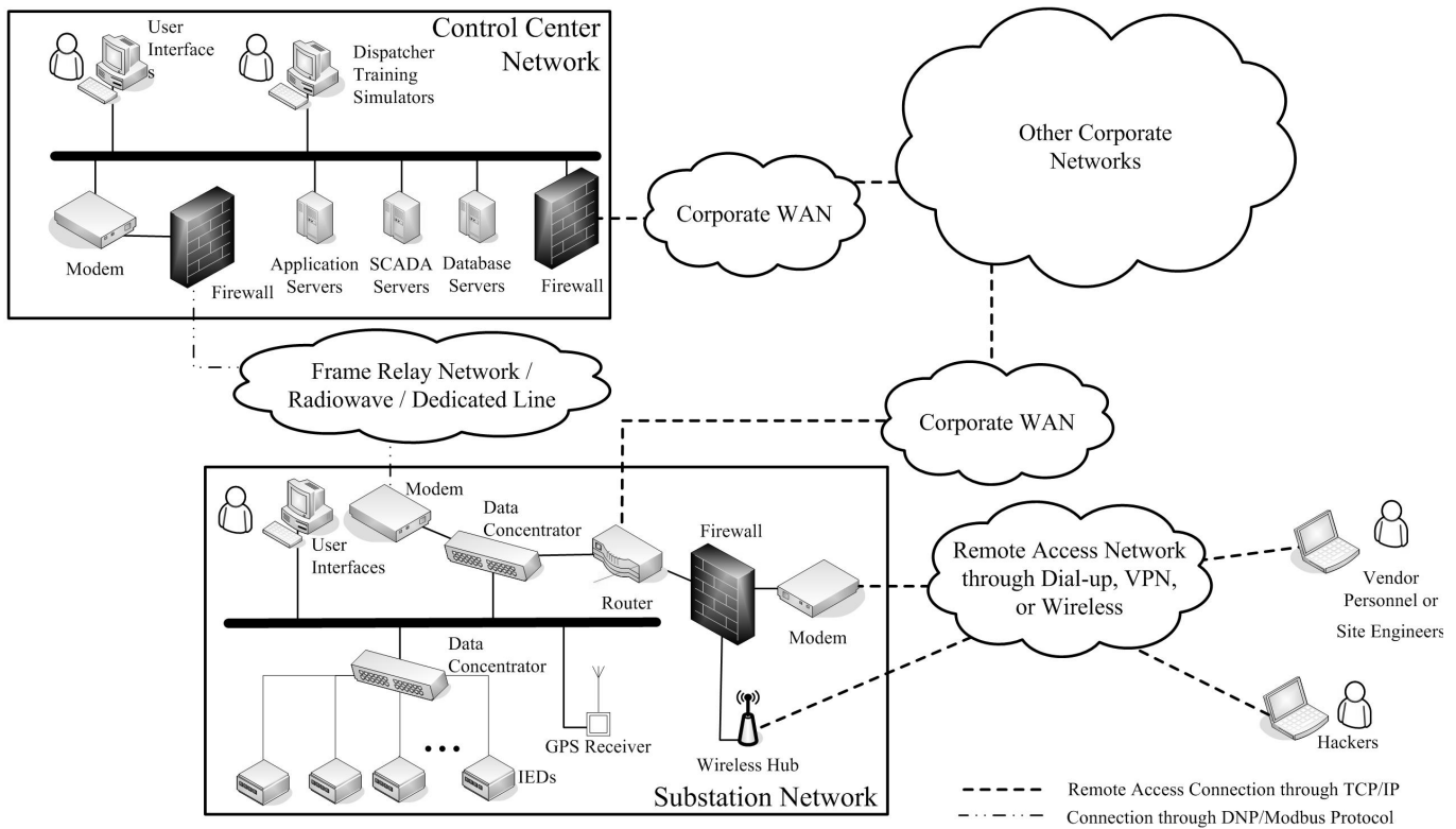
Fig. 1. Cyber Network Environment of a Control Center
