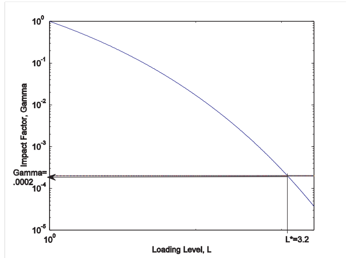
Fig. 9. Impact Factor vs. Loading Level
