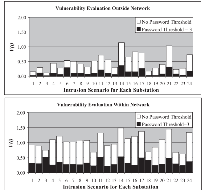
Fig. 11. Scenario Vulnerability Indices for Each Intrusion Scenario
