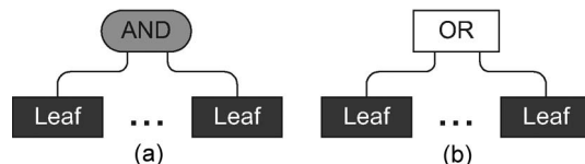
Fig. 2. Attack leaves with “AND” and “OR.” (a) Attack leaf with logic operator “AND.” (b) An attack leaf with logic operator “OR.”
